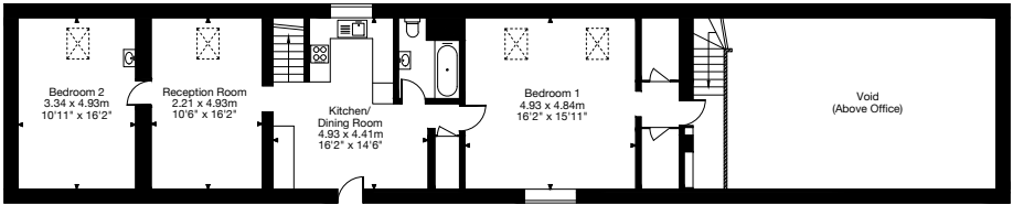
First Floor (Annexe)
