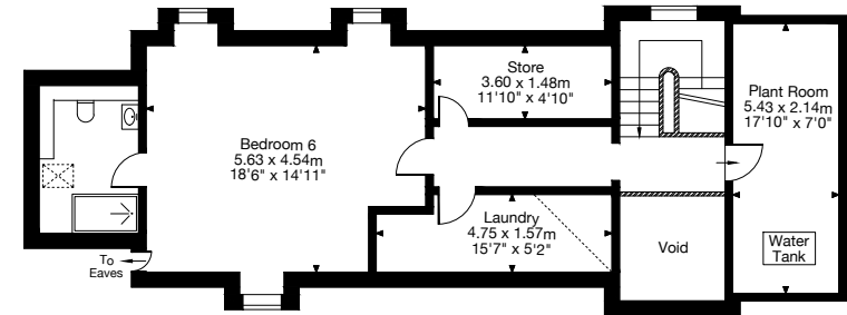
Second Floor
