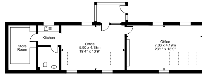
Office
