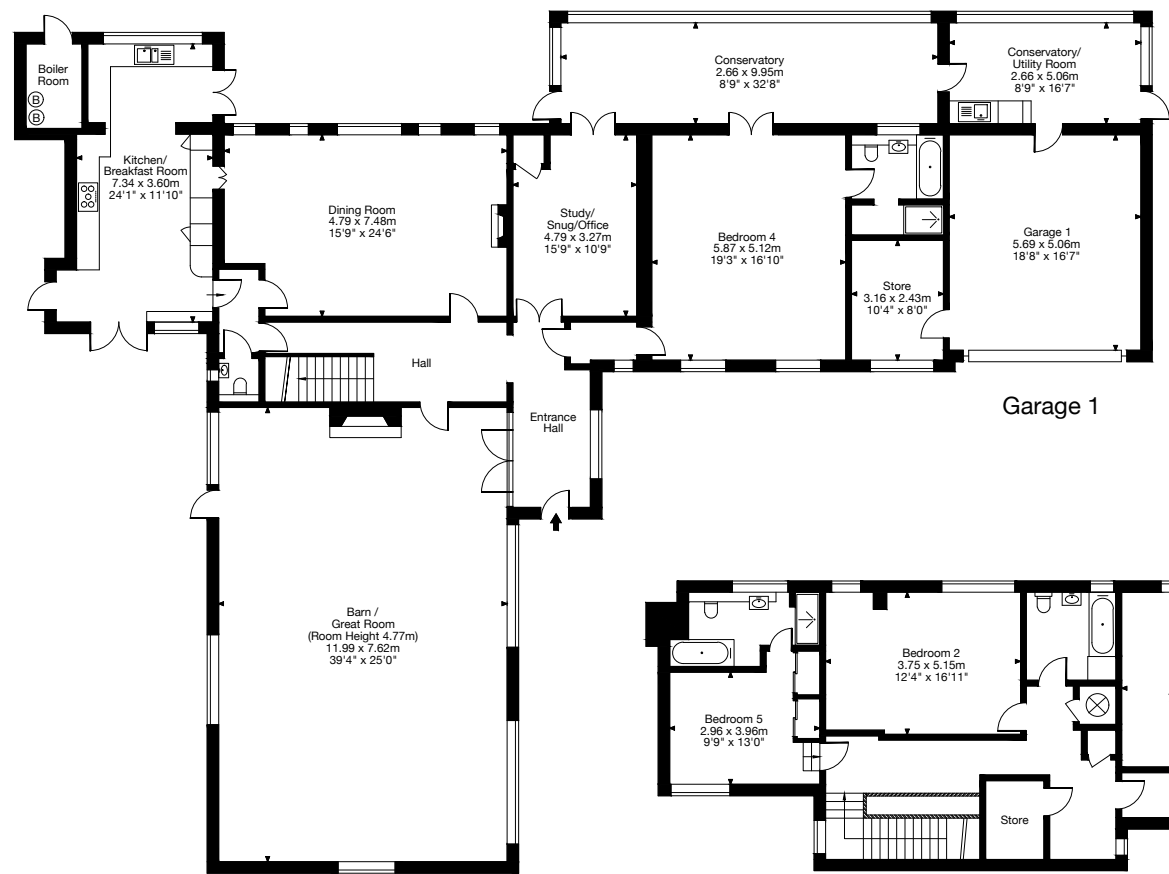
Ground Floor Main House
