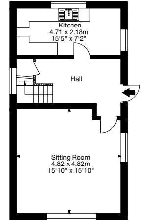
Ground Floor Cottage
