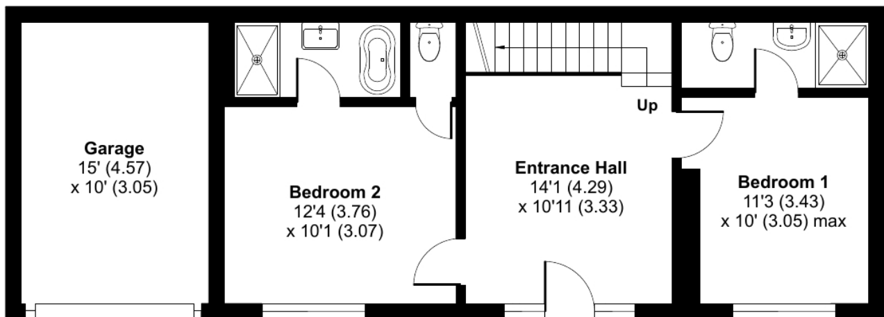
ROCKTON MEWS GROUND FLOOR
